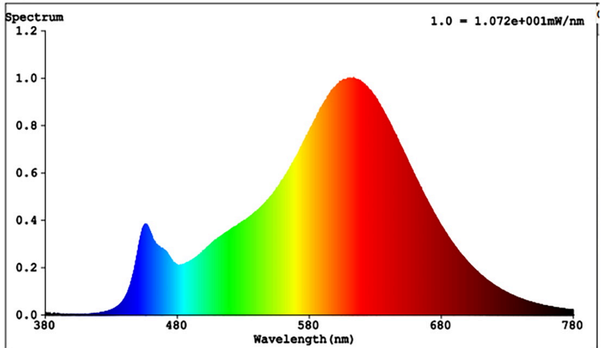
Spectral Distribution
